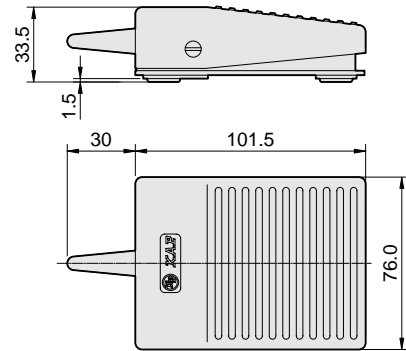
Thermoplastic Miniature Foot Switch
