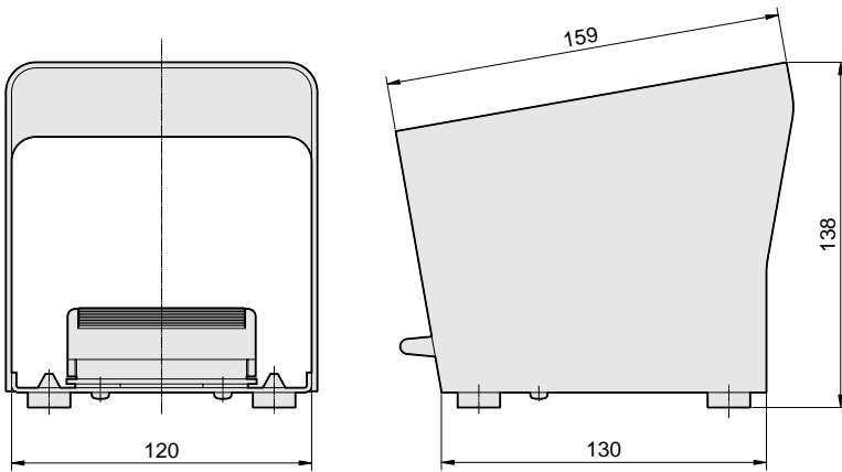
Metal Protection Cover to Thermoplastic or Metal Miniature Foot Switch
